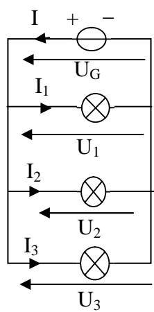
Circuit n°2
