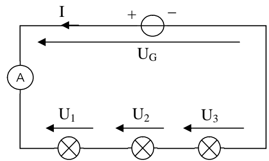
Circuit n°1
